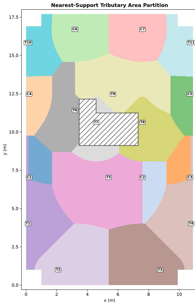
Figure 3. Nearest-support tributary-area partition.
