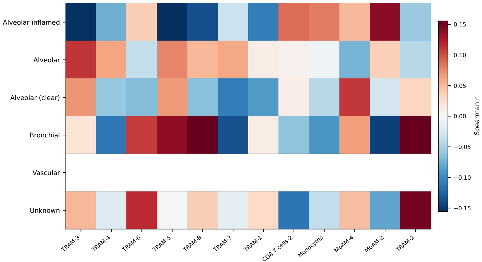
Figure 15 — BAL × H&E Cross-Modal Correlation (Spearman r , n=94 paired; * FDR<5%)
