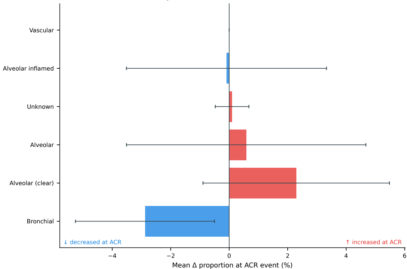
Figure 16 — H&E Fingerprint at ACR Episode (n=31 paired ACR+/ACR- consecutive visits)
