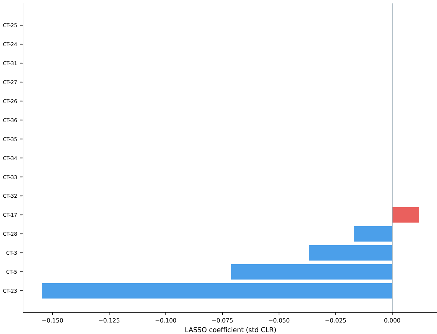
Figure 23 — CT scan: Multi-cluster CLR Signature (LASSO + RF) ACR — LASSO (AUC=0.60) ASSO: L1-penalised logistic; RF: Gini impurity; CLR-normalised inputs) ACR — RF (AUC=0.65)
