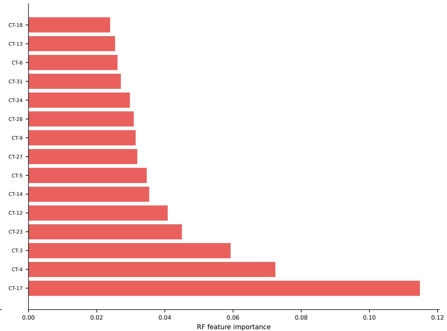
Figure 23 — CT scan: Multi-cluster CLR Signature (LASSO + RF) ACR — LASSO (AUC=0.60) ASSO: L1-penalised logistic; RF: Gini impurity; CLR-normalised inputs) ACR — RF (AUC=0.65)
