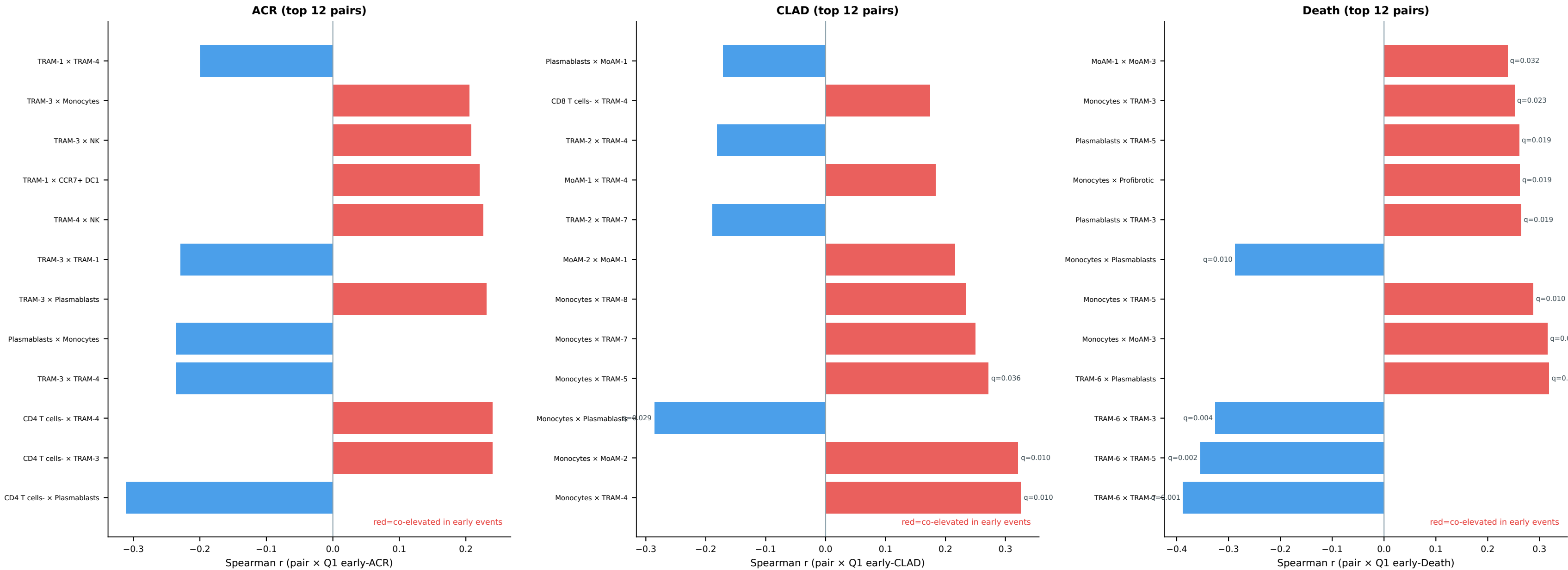
Figure 24 — BAL scRNA: Cluster Pairs Co-elevated in EARLIEST Events (Q1) (CLR product Spearman r vs Q1-flag; Q1=earliest 25%% of events, ref=Q4+censored)
