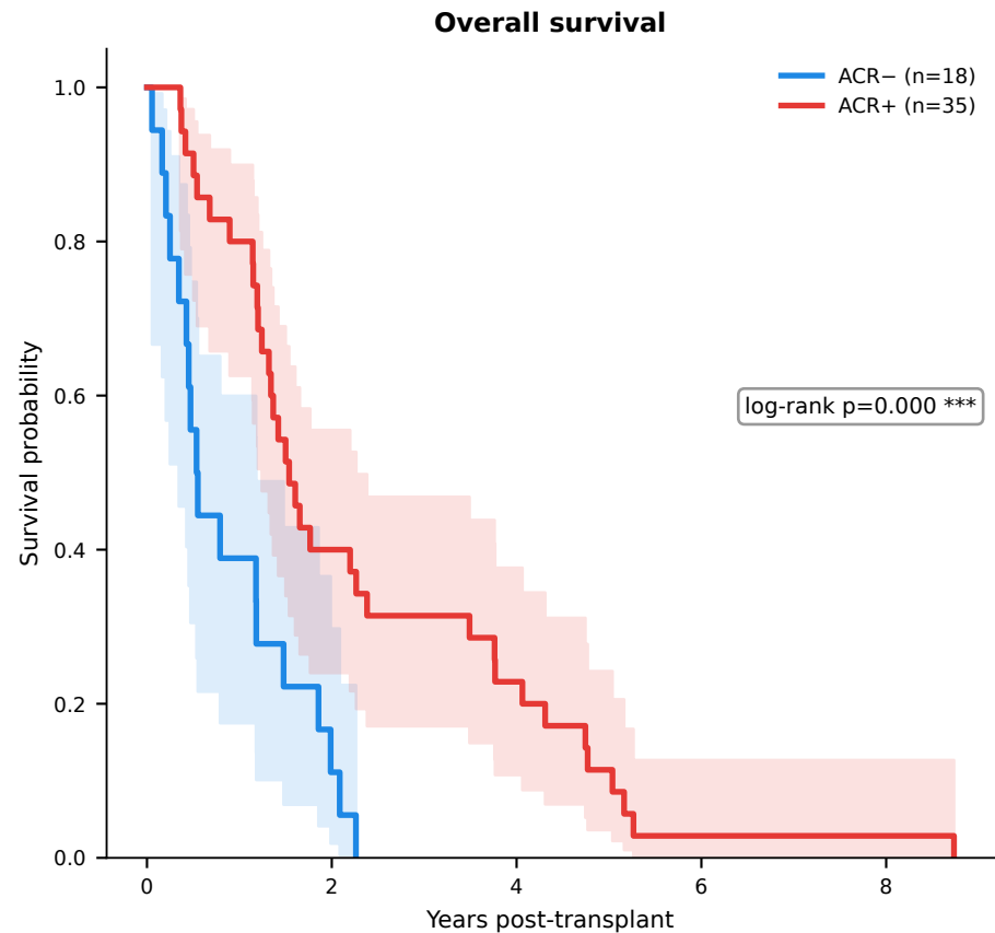
Figure 6 — Survival by ACR Status
