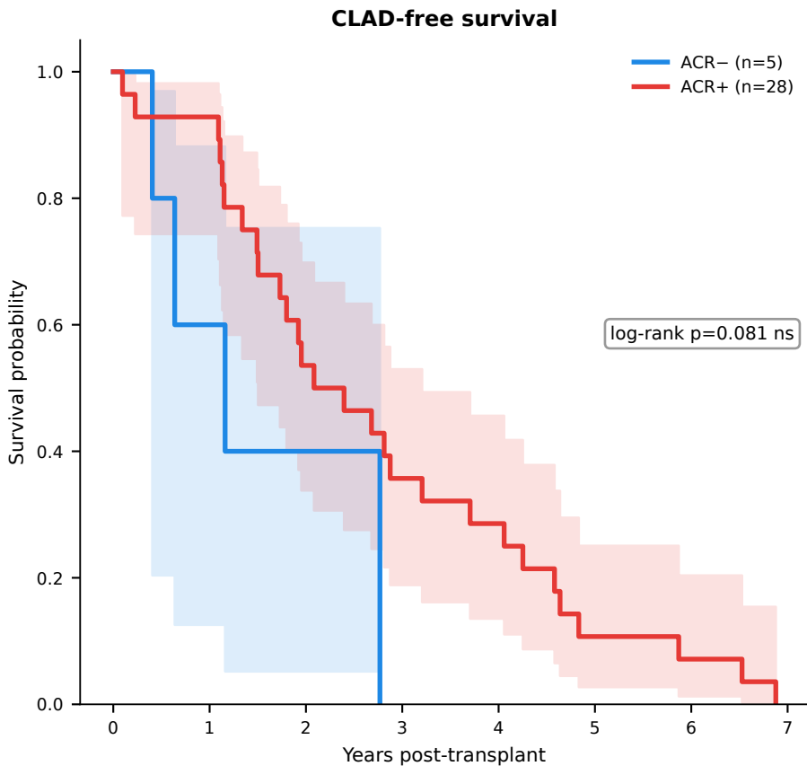
Figure 6 — Survival by ACR Status
