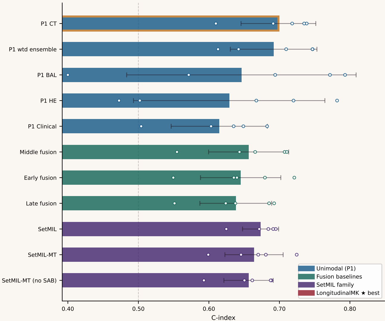
Death survival (C-index)
