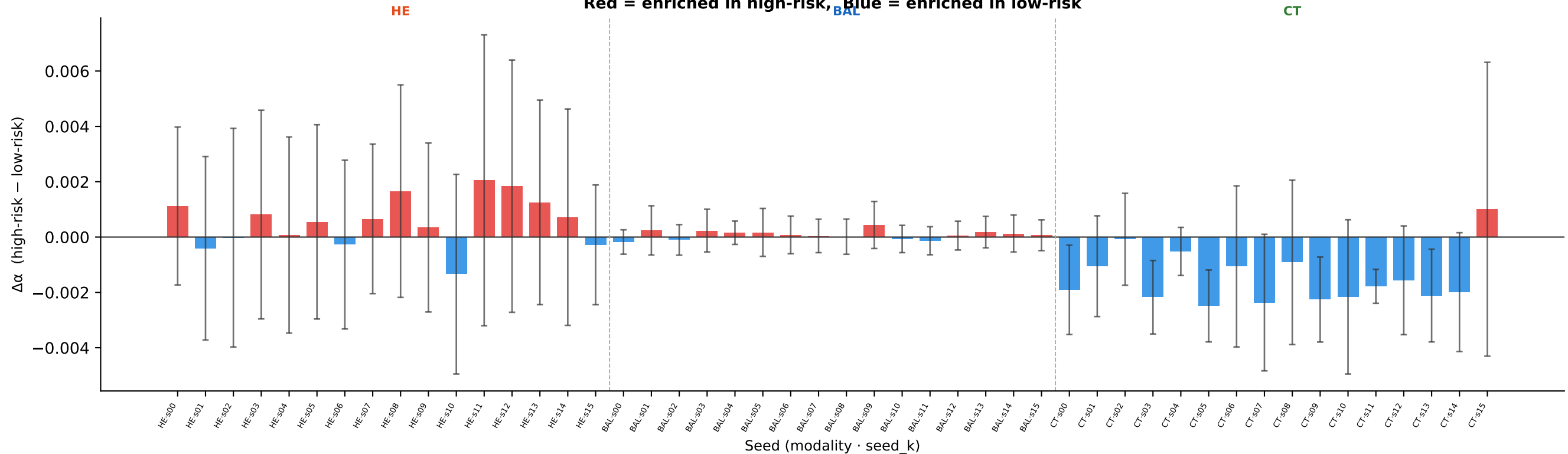
CLAD — Seed attribution \Delta\alpha (mean \pm std, n=5 splits) Red = enriched in high-risk, Blue = enriched in low-risk
