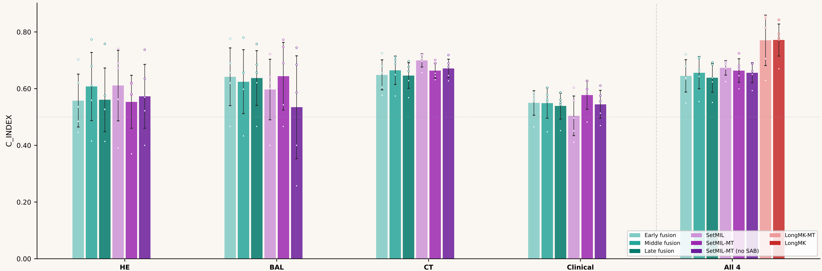
Modality contribution — Death survival (C-index)
