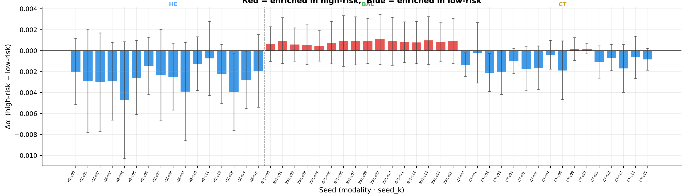
ACR Classification — Seed attribution \Delta\alpha (mean \pm std, n=3 splits) Red = enriched in high-risk, Blue = enriched in low-risk
