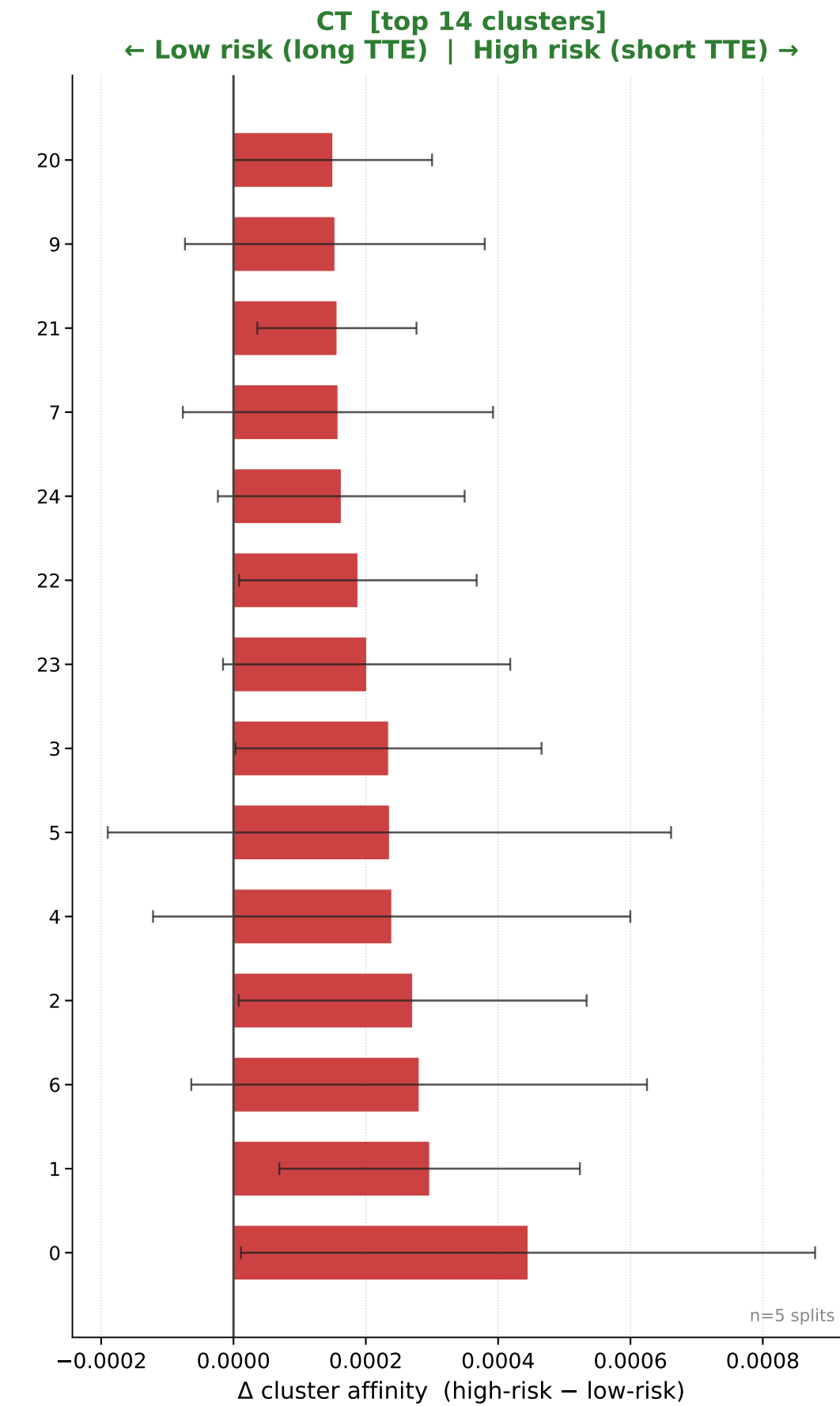
CLAD Survival (time to CLAD onset) Model: set_mil_mt [C-index 0.563 +/- 0.080] | Cluster attribution \Delta affinity (mean \pm s.d., 5 splits)
