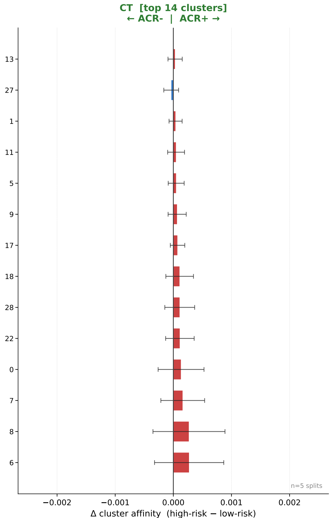
ACR Classification (ACR+ vs ACR-) Model: set_mil_mt_no_sab [BACC 0.623 +/- 0.034] | Cluster attribution Δ affinity (mean ± s.d., 5 splits)
