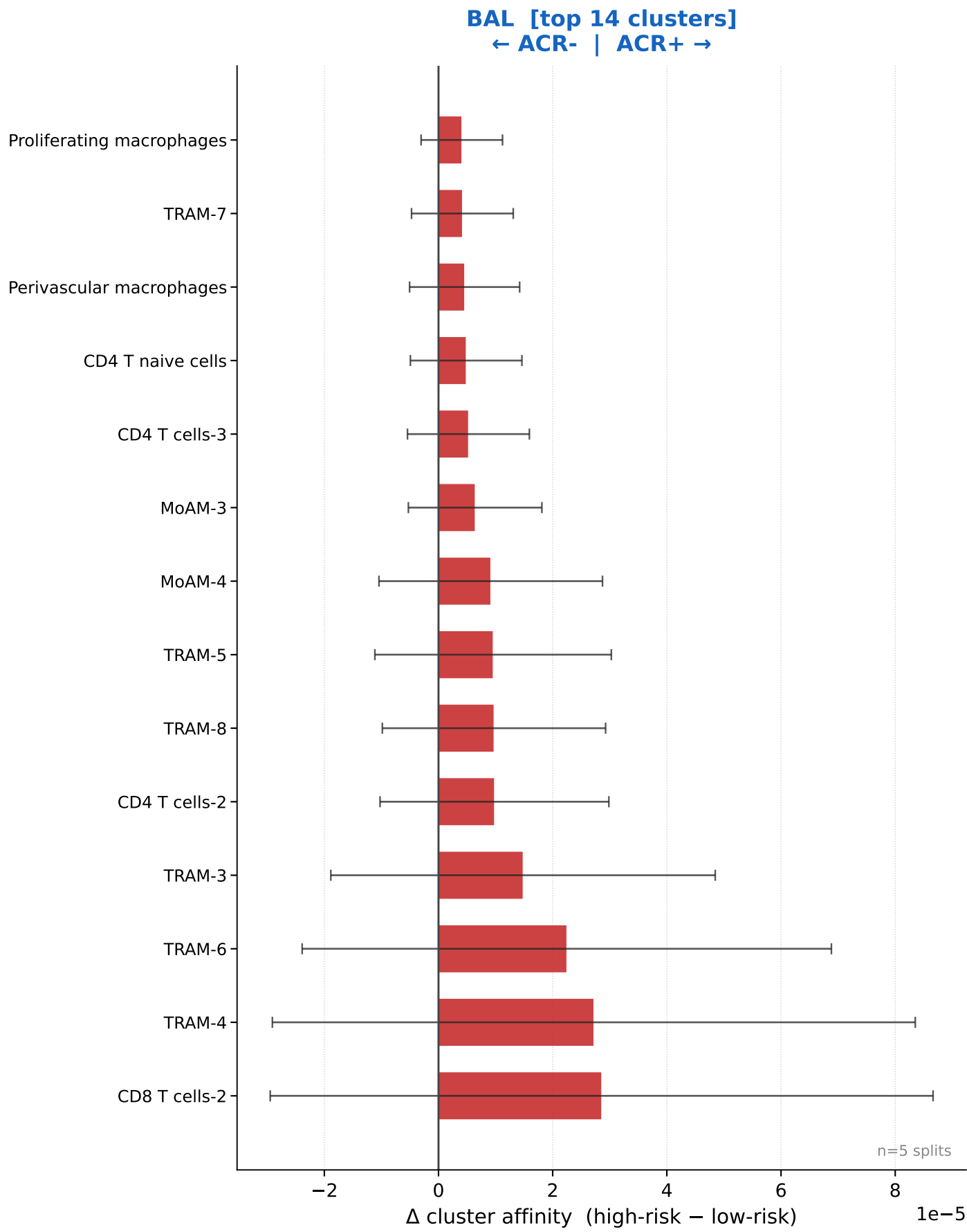
ACR Classification (ACR+ vs ACR-) Model: set_mil_mt_no_sab [BACC 0.623 +/- 0.034] | Cluster attribution \Delta affinity (mean \pm s.d., 5 splits)
