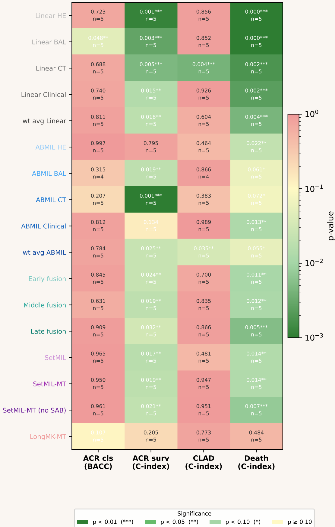
LongMK vs. all models — one-sided paired t-test p(LongMK > other), n = number of valid paired splits
