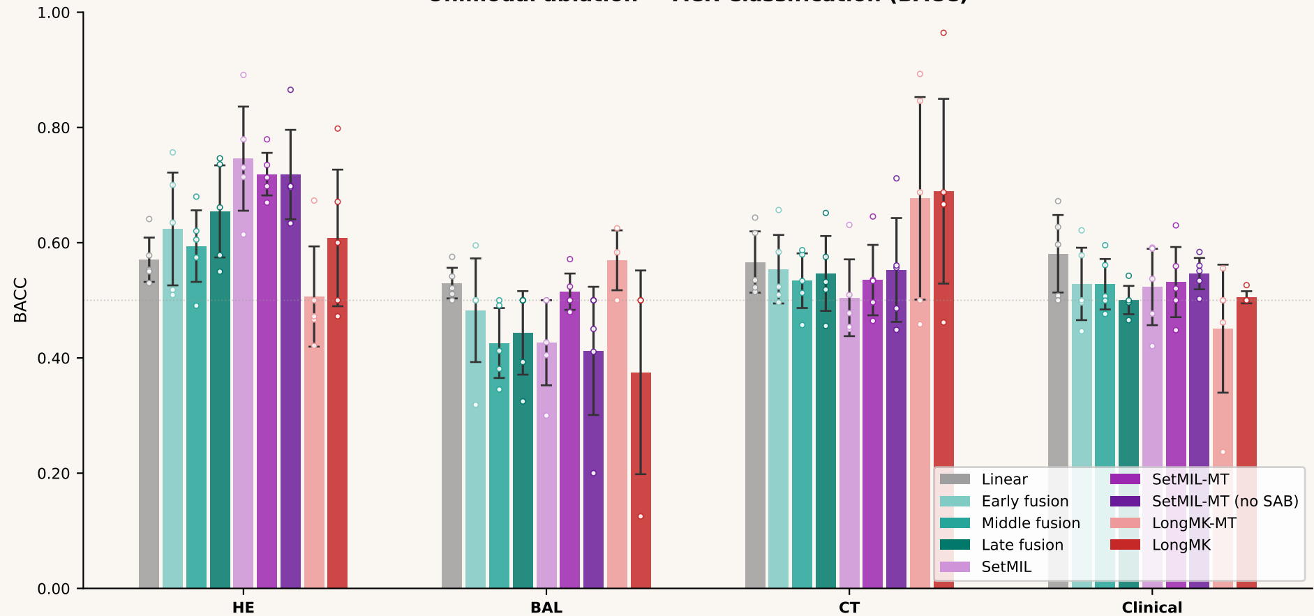
Unimodal ablation — ACR Classification (BACC)
