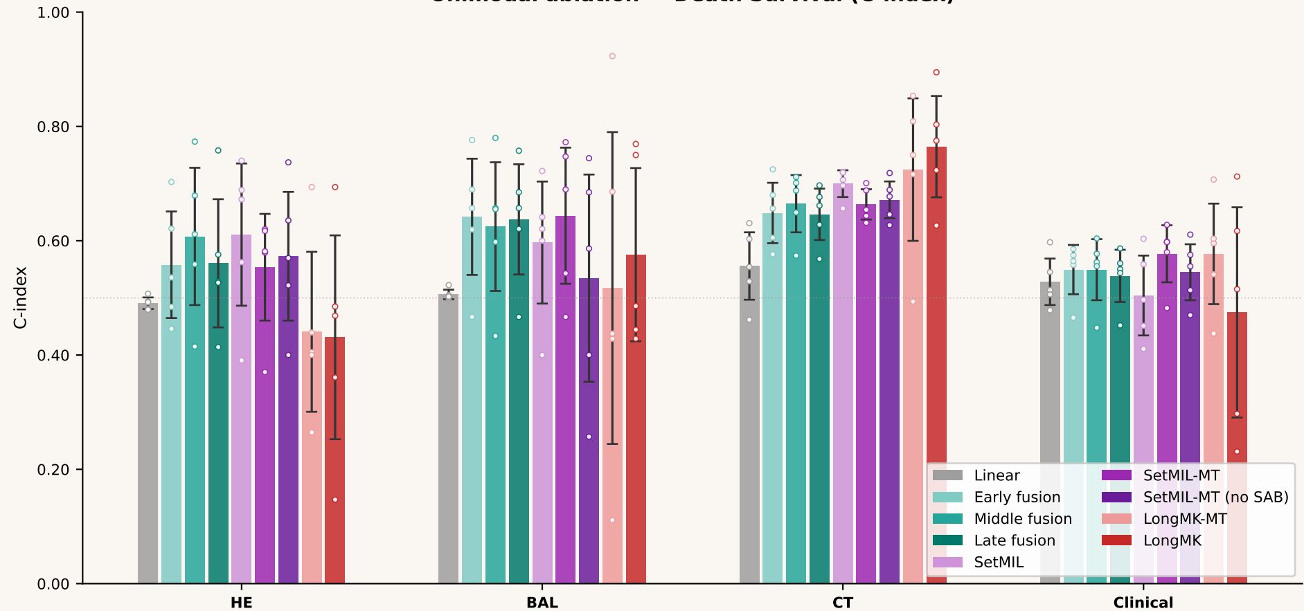
Unimodal ablation — Death Survival (C-index)
