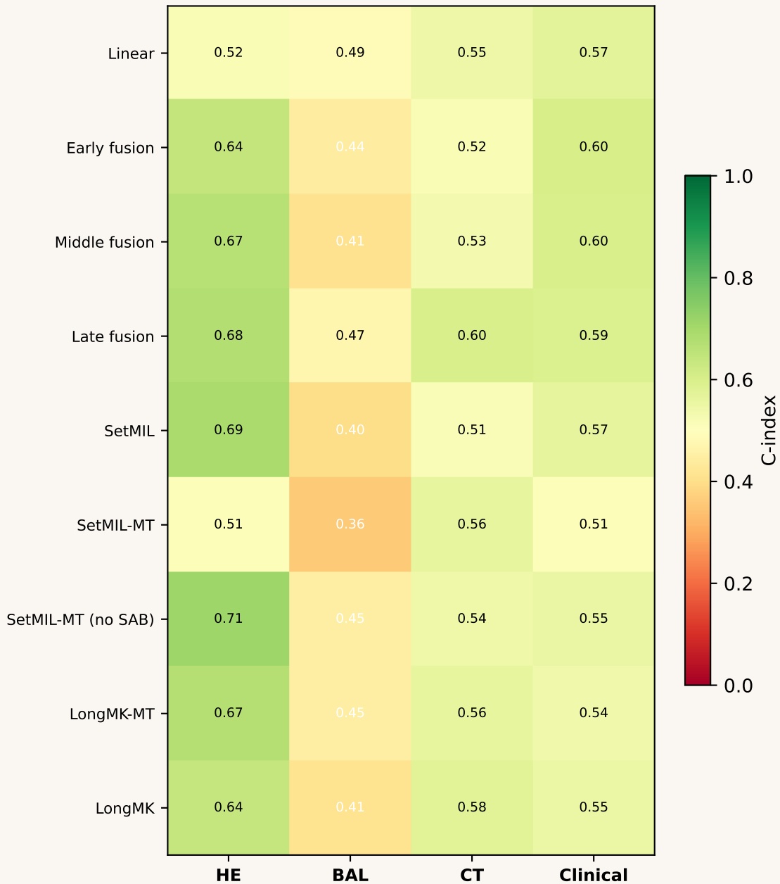
Unimodal ablation heatmap — ACR Survival (C-index)
