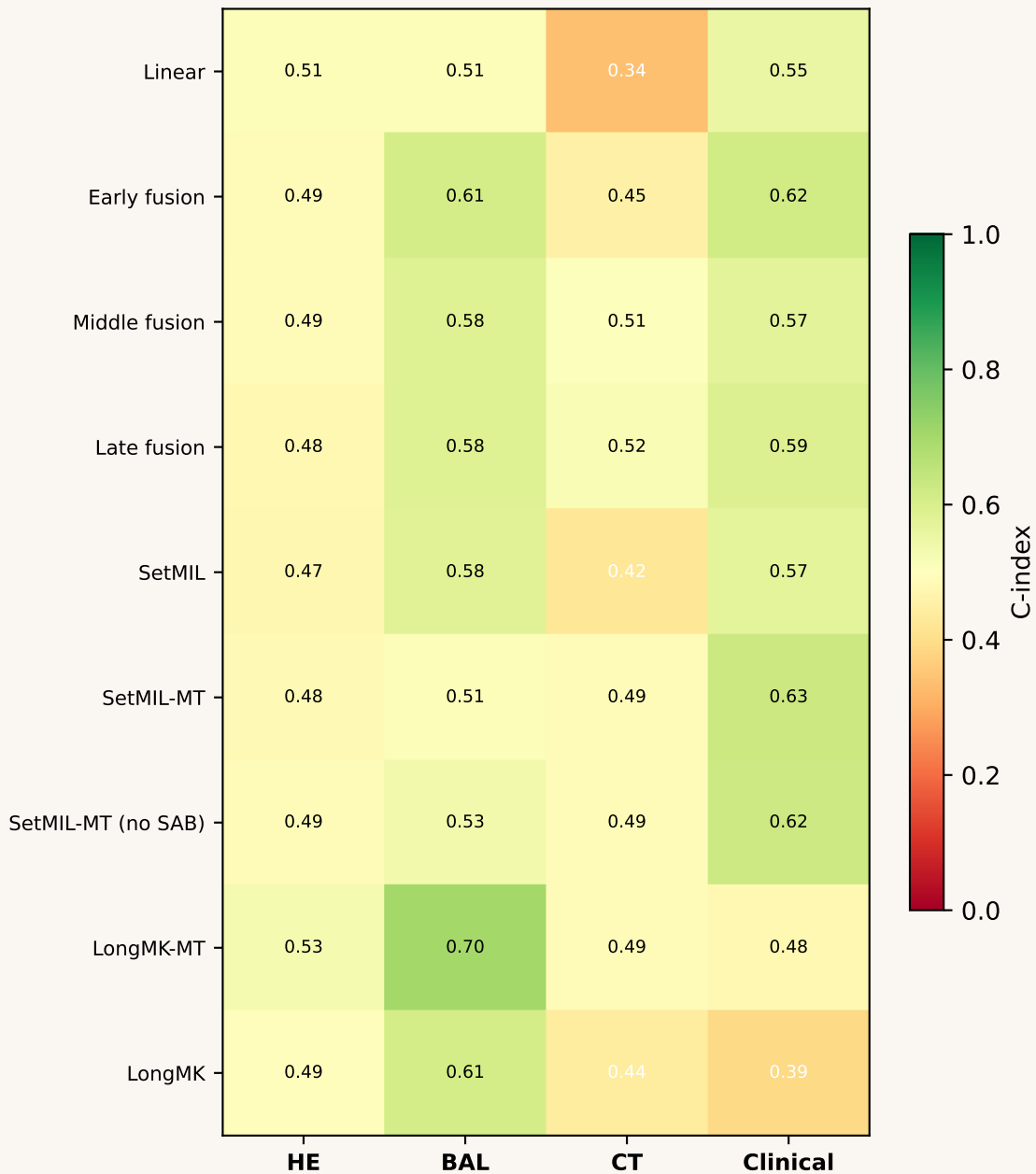
Unimodal ablation heatmap — CLAD Survival (C-index)
