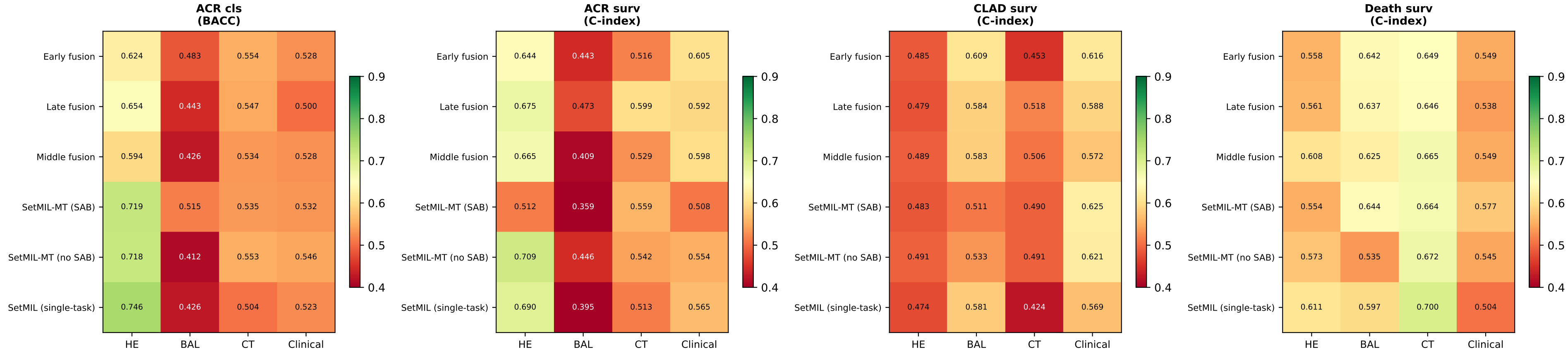
Unimodal ablation heatmap (mean across splits)
