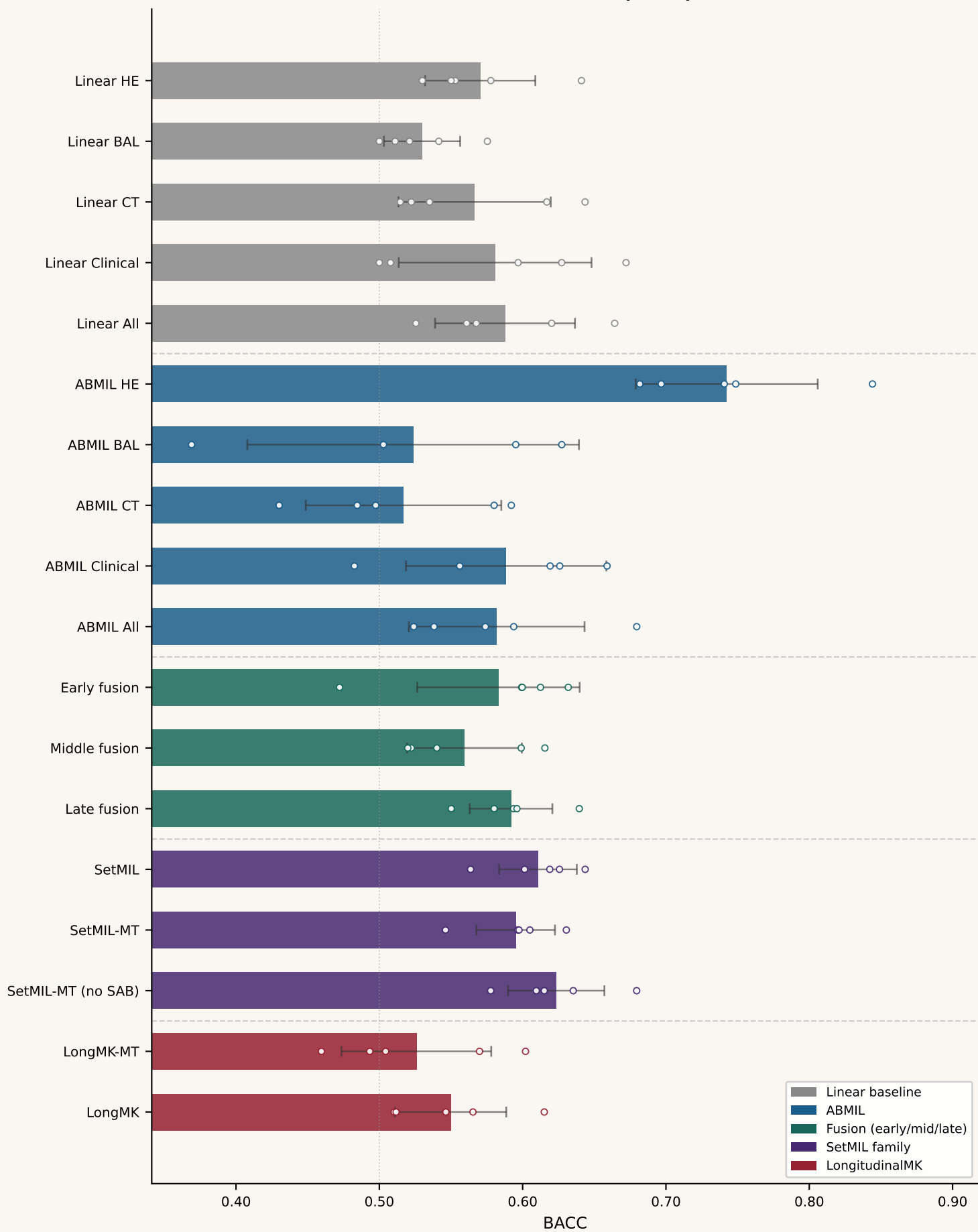
ACR classification (BACC)
