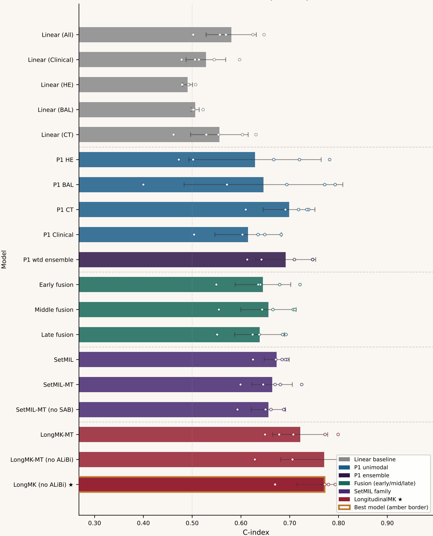
Death survival (C-index)
