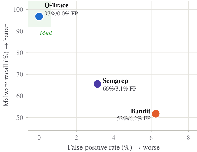
Fig. 6. Recall vs. false-positive quadrant. The ideal tool sits in the top-left corner (high recall, low FP). Q-Trace occupies it; Semgrep and Bandit trade recall for a non-zero false-positive rate. Each tool is plotted at its own recommended CI gate.
