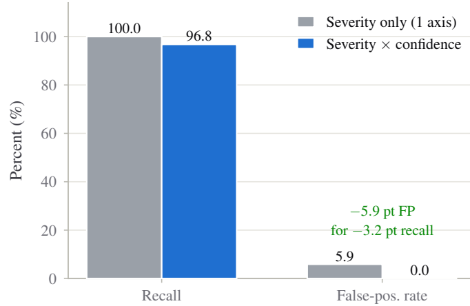
Fig. 4. Confidence-axis ablation. Removing the confidence axis (severity-only gate) recovers one detection but introduces two false positives (5.9% FP). The two-axis gate trades 3.2 points of gate-recall for the elimination of all false positives—the trade that governs real-world adoption.
