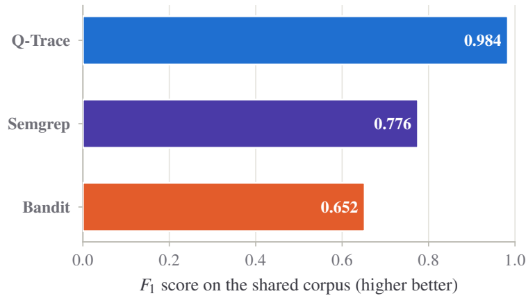
Fig. 8. F_1 on the shared code corpus. The gap is driven jointly by higher recall and zero false positives.
