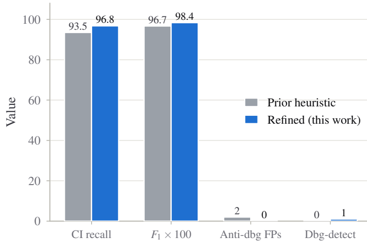
Fig. 5. Effect of the evidence-based anti-analysis refinement. The refined engine improves gate-recall and F_1 while removing false positives and adding debugger-detection coverage. Prior-version values were measured on the same corpus at the start of this work.
