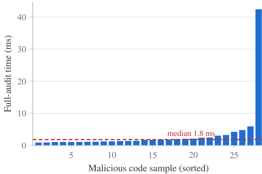
Fig. 12. Per-sample full-audit latency (28 malicious code samples, sorted). The dashed line marks the median; the single tall bar is cold-start warm-up. Steady-state analysis is sub-2 ms.
