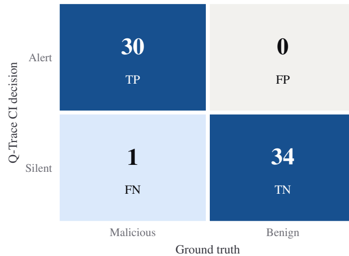
Fig. 9. Q-Trace confusion matrix over all 65 samples (TP=30, FN=1, FP=0, TN=34). The single false negative is the SSRF case of Section XI-D.
