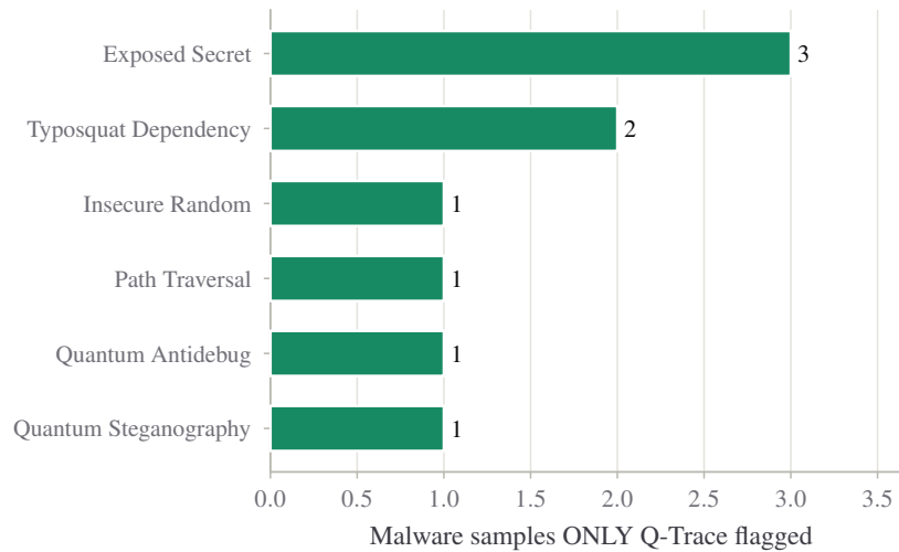
Fig. 11. Malware caught only by Q-Trace, by threat class. These are the stealth and supply-chain classes for which single-file pattern matchers have no rule class.
