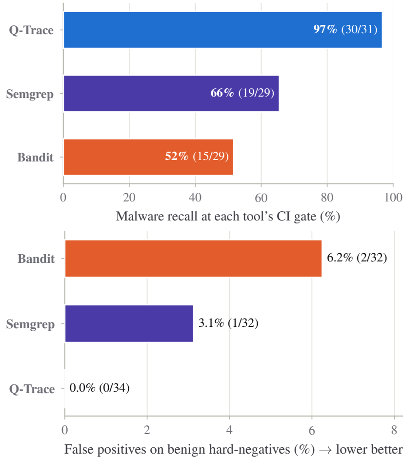
Fig. 7. Malware recall (top) and false-positive rate (bottom) by tool at each tool's CI gate. Q-Trace holds 0% FP; the false positives raised by Bandit and Semgrep are precisely the everyday-code patterns that drive alert fatigue.
