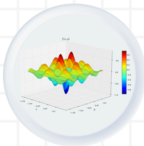
Simulated Annealing
