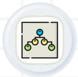
Hierarchical Clustering
