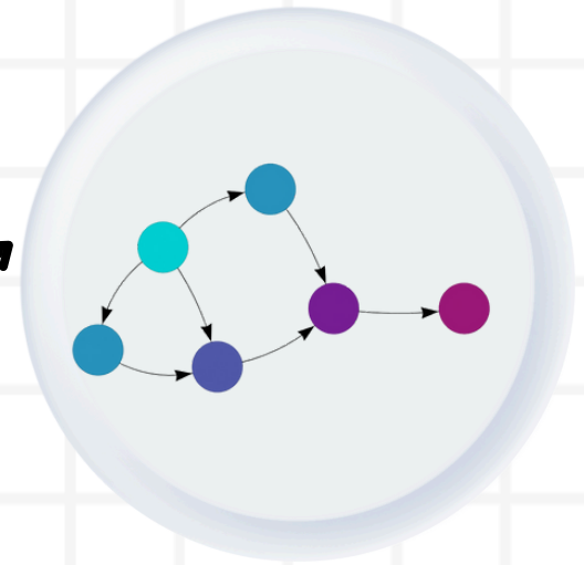
Bayesian Networks
