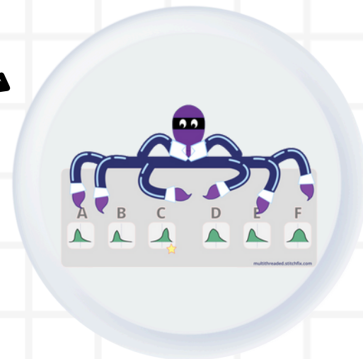
Multi-Armed Bandit
