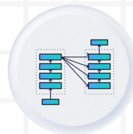
Transformers
