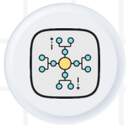
DBSCAN
