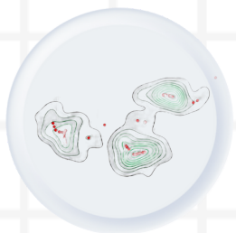
Spectral Clustering
