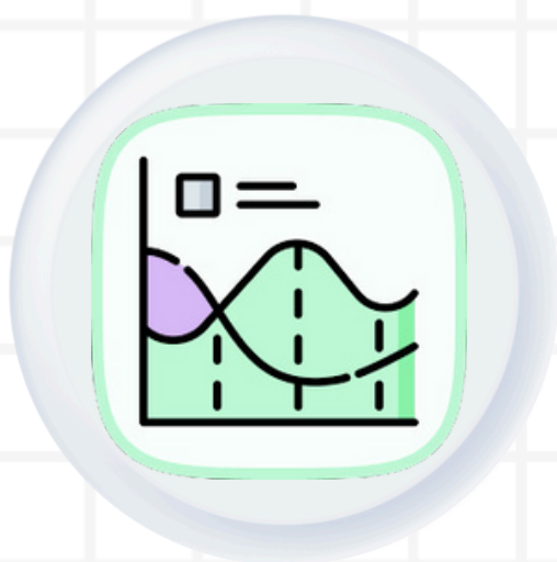
Gaussian Processes
