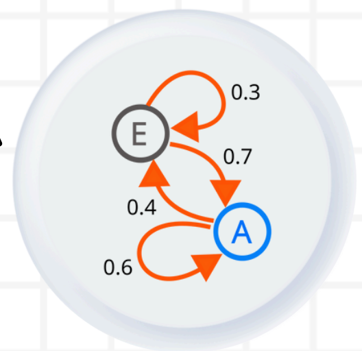
Markov Chains
