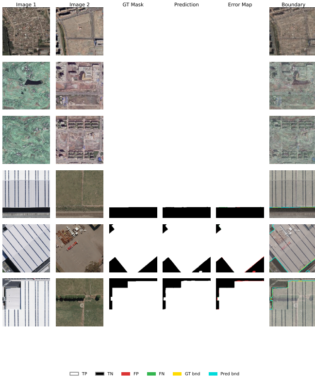
Fig. 1. Qualitative boundary results on DSIFN-CD (A6 full model). Each row: I_1 , I_2 , GT, prediction, error map (white = TP, black = TN, red = FP, green = FN), boundary overlay (yellow = GT bnd, cyan = pred bnd).
