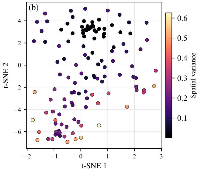
Channel-wise D_I embedding
