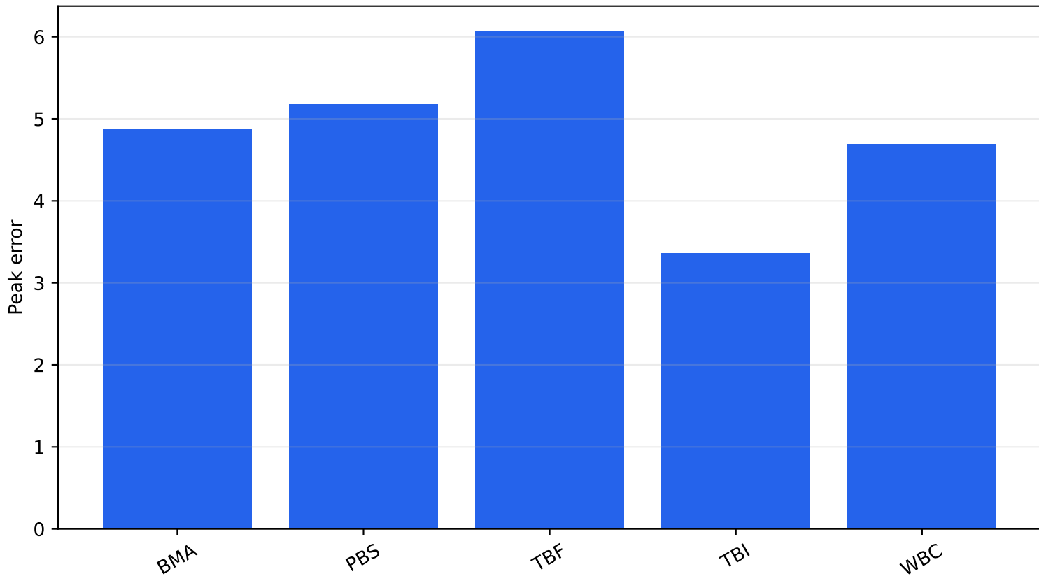
Dataset-wise performance
