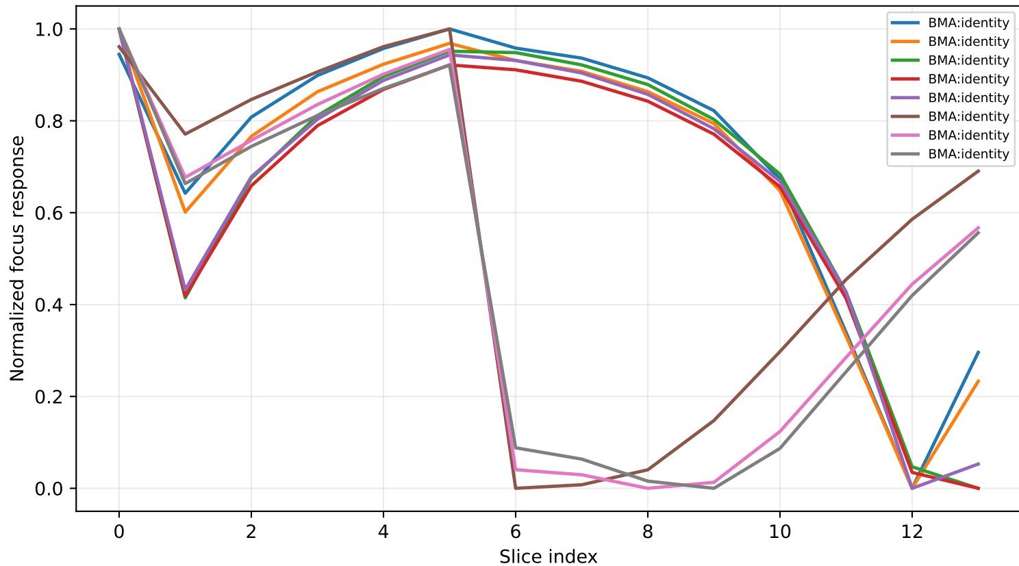
Representative normalized focus curves
