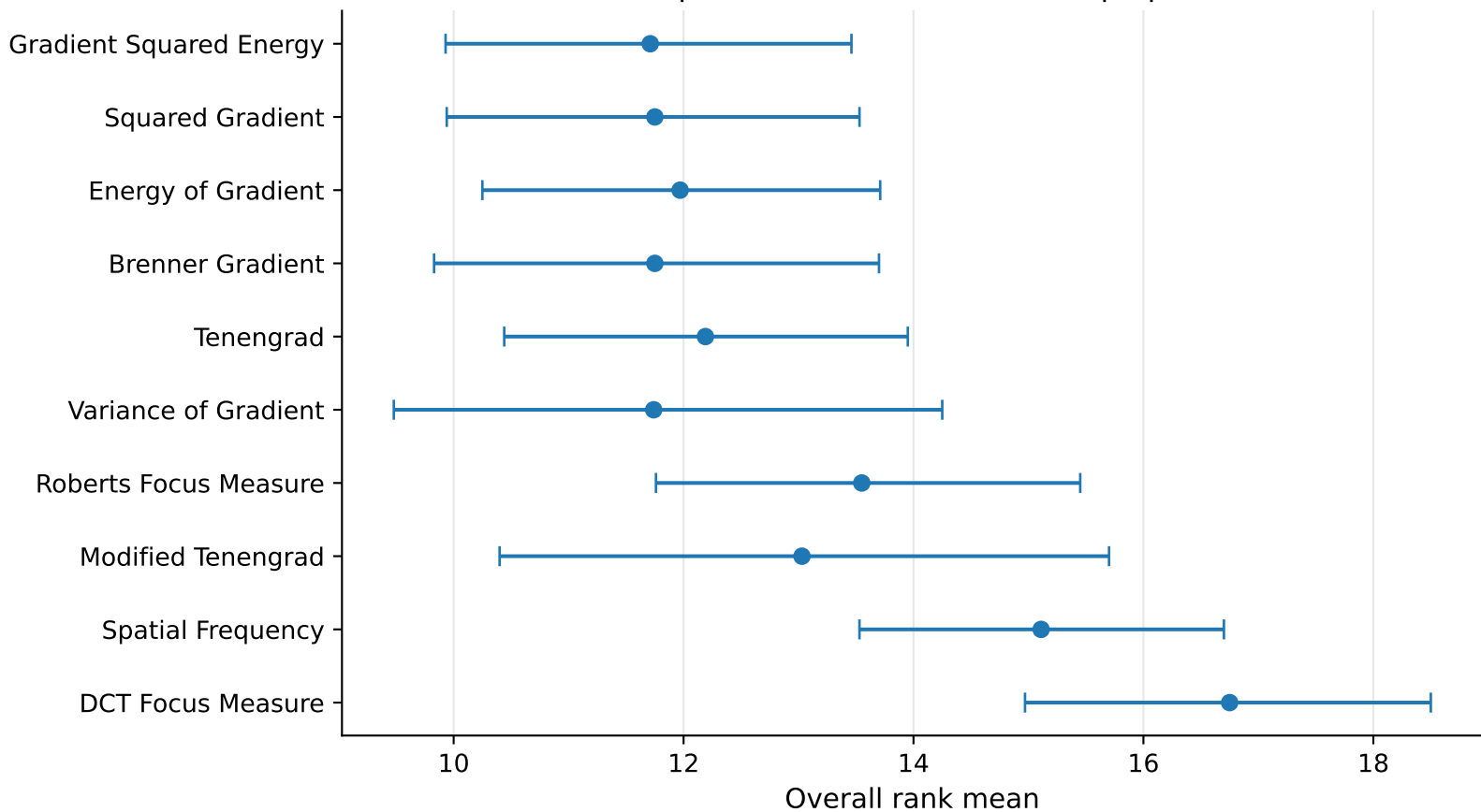
Bootstrap confidence intervals for top operators
