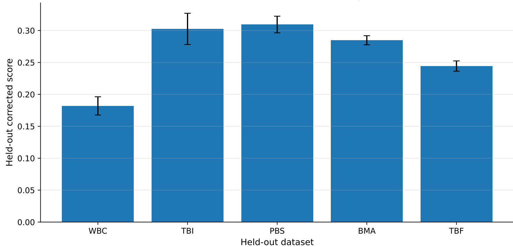
Leave-one-dataset-out GP summary
