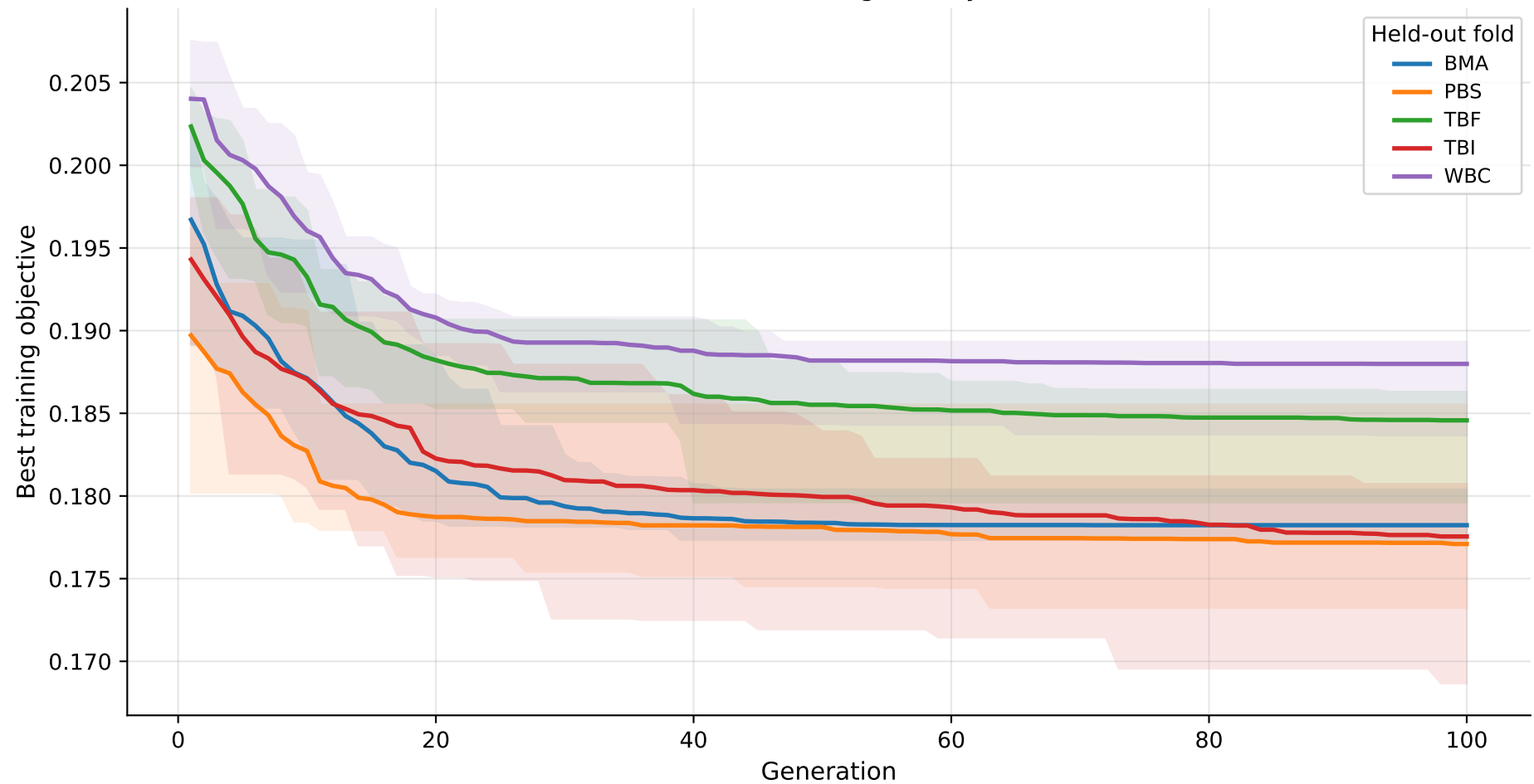
Generation-wise GP convergence by held-out fold
