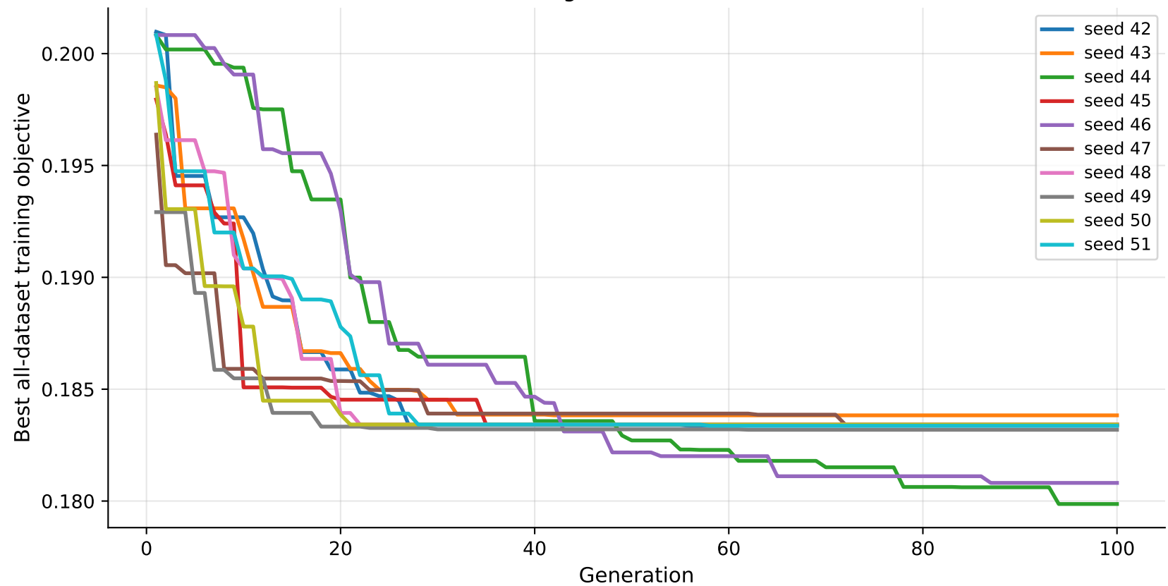
Generation-wise convergence of the final all-dataset GP refit
