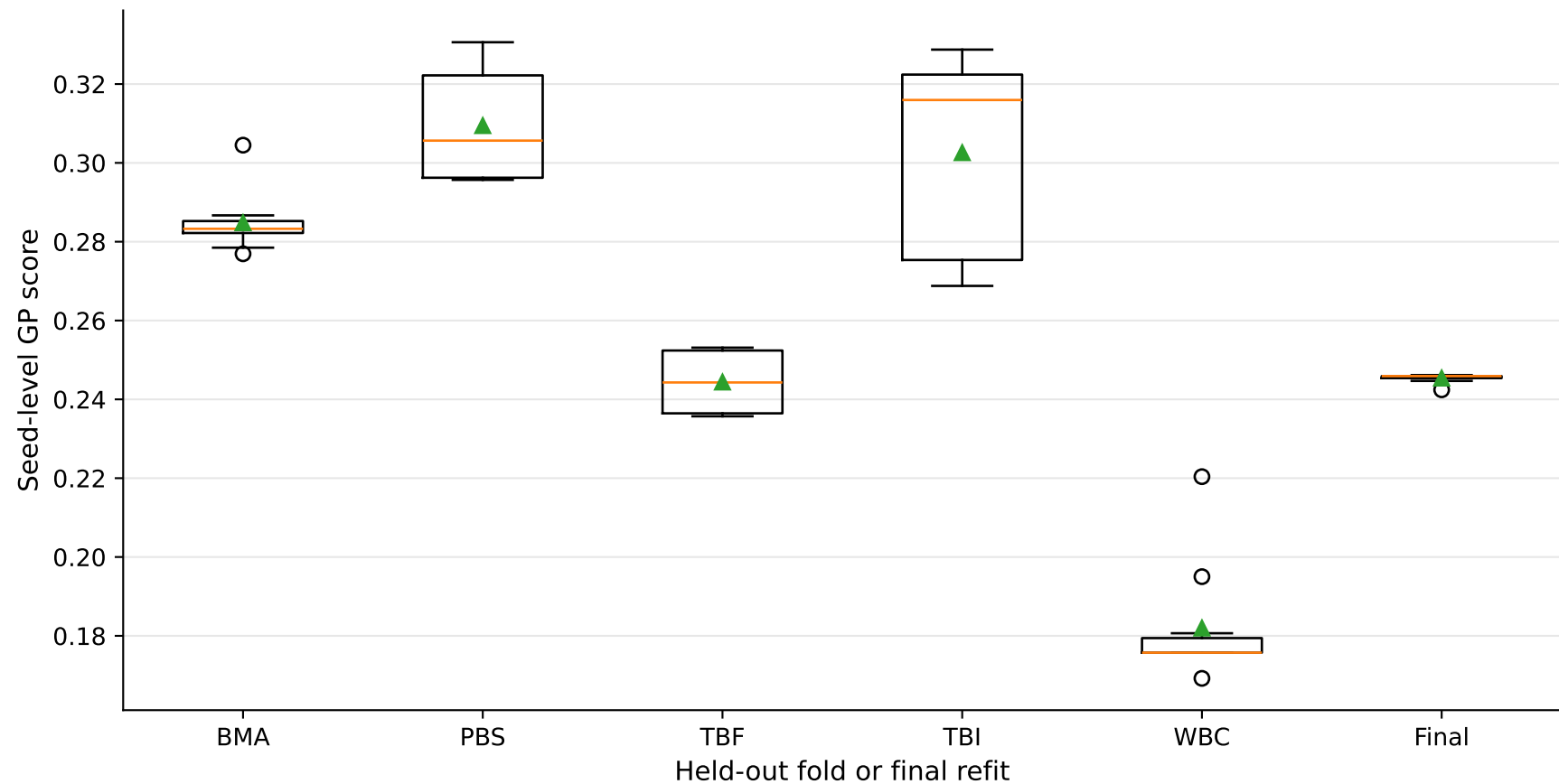
Seed-wise GP score distribution across LODO and final refit
