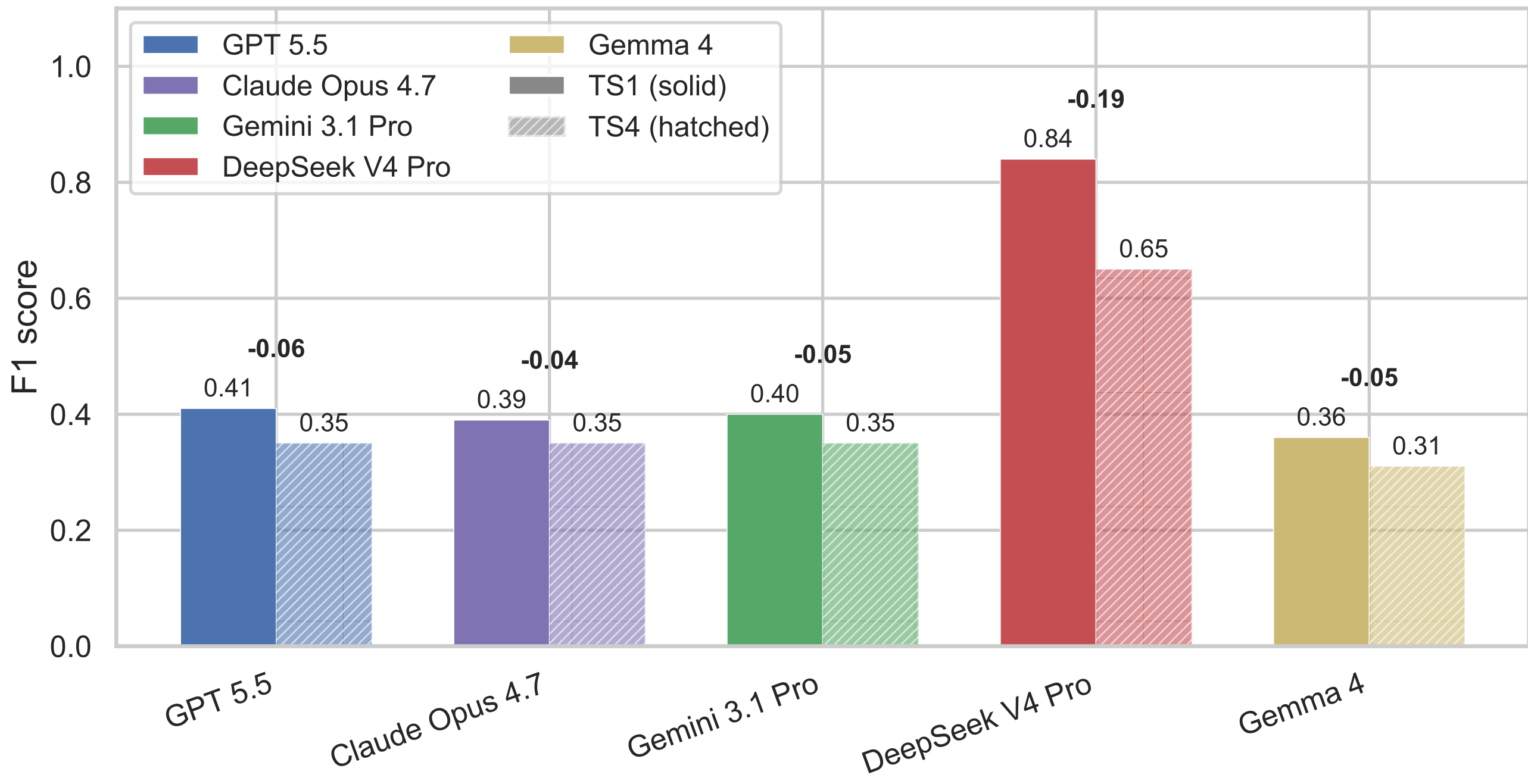
F1 score comparison between TS1 and TS4
