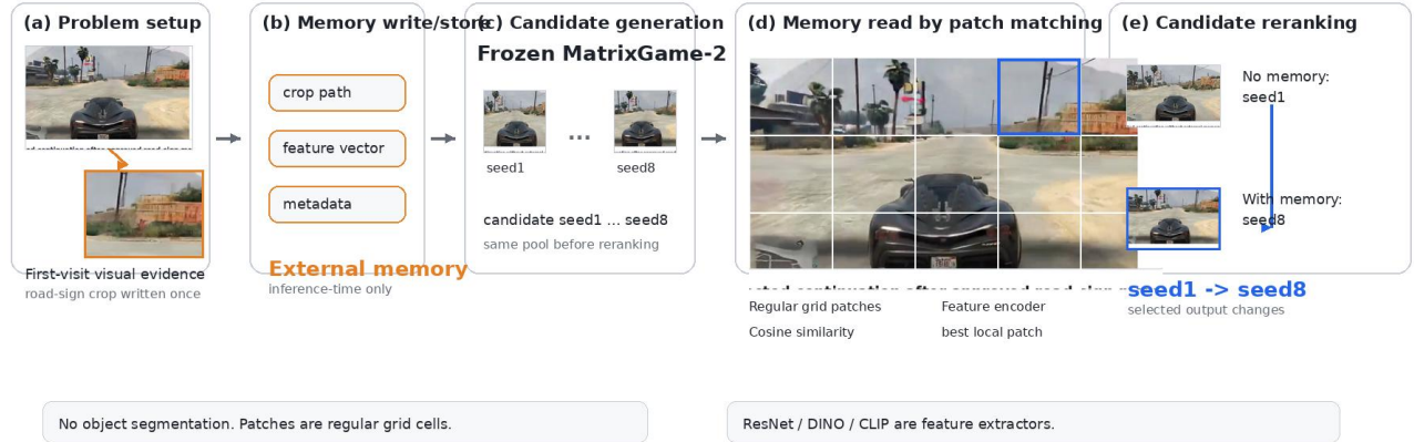
Figure 1. Overview of our Stage C external memory reranking pipeline. MatrixGame-2 is kept frozen. The memory module writes first-visit visual evidence, reads it through patch-level feature matching on regular grid patches, and reranks candidate videos.
