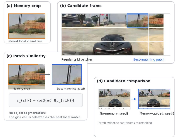
Figure 2. Patch-level memory read. A stored memory crop is compared with regular-grid patches from candidate frames. The best-matching patch provides local evidence for memory-guided reranking.
