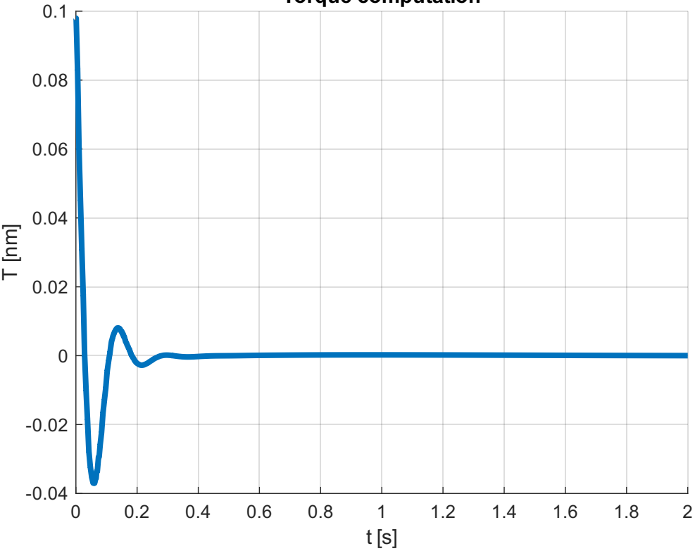
Torque computation
