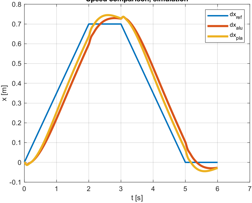
Speed comparison, simulation
