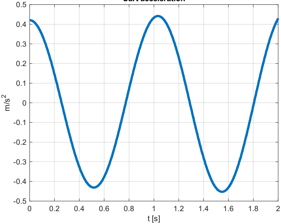
Cart acceleration
