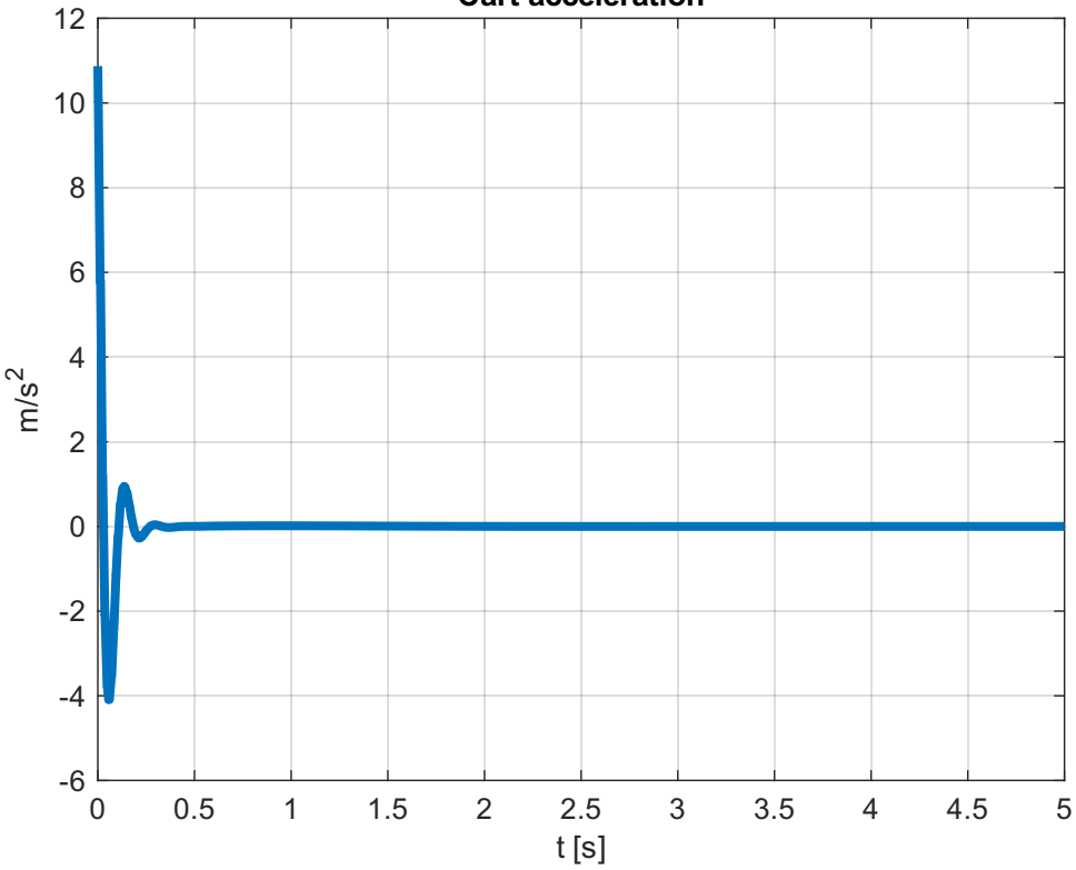
Cart acceleration
