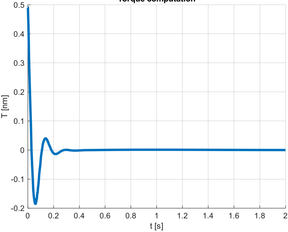
Torque computation
