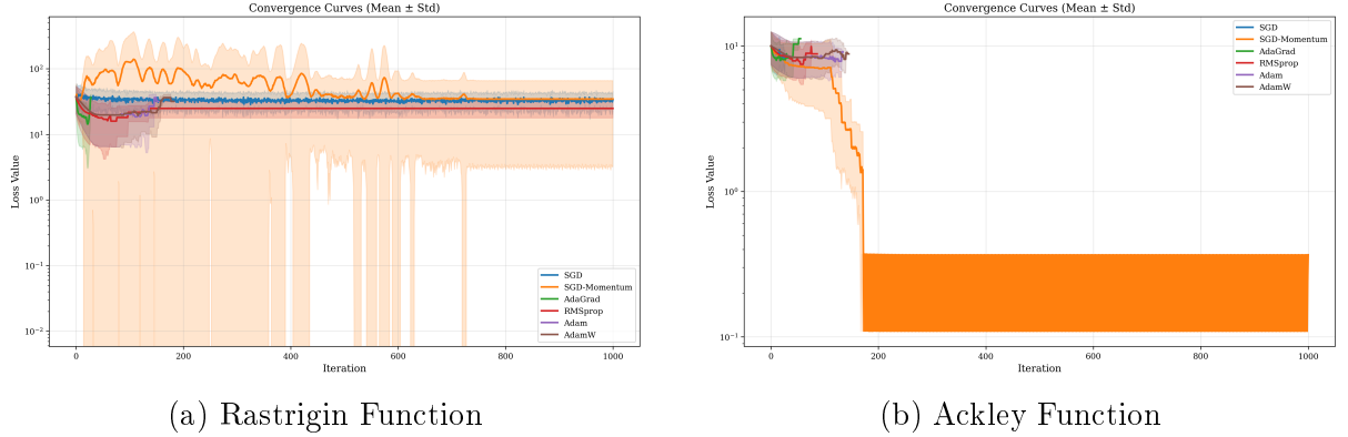
Figure 3: Convergence curves showing loss vs. iteration (log scale). Lines show mean values, shaded regions show \pm 1 standard deviation.
