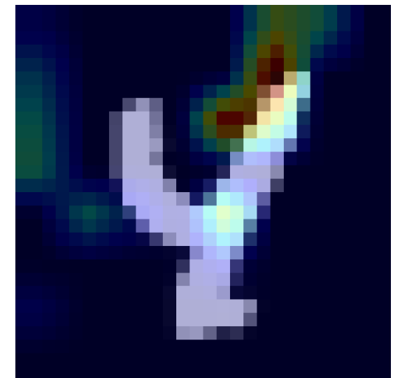
Feature Difference recons_z2-z2
