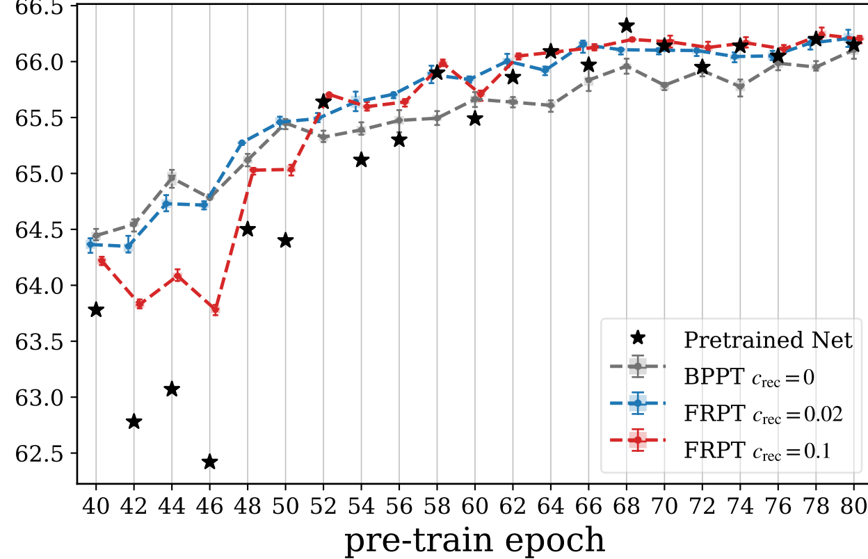
mean testacc (%)
