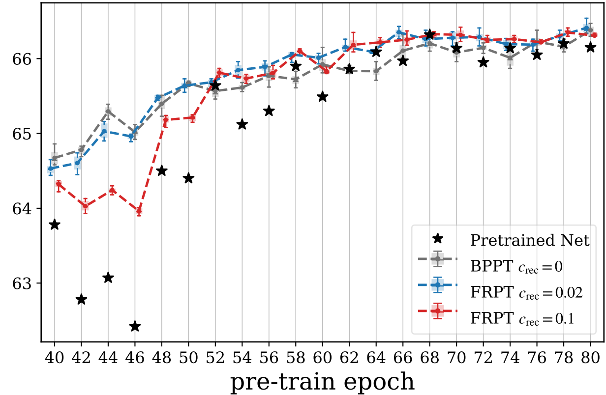
best testacc (%)
