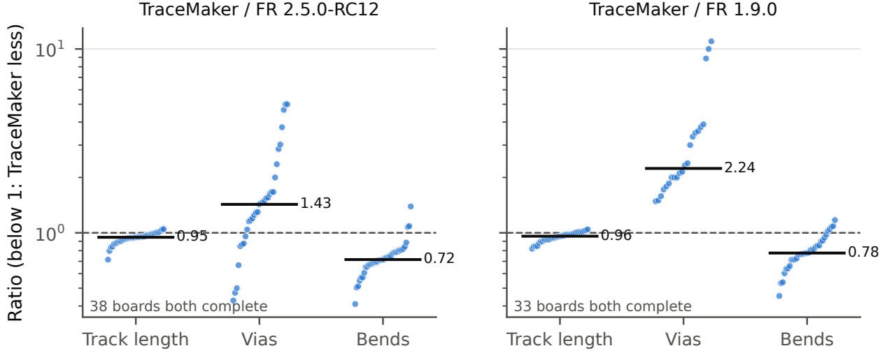
Figure 12: Layout quality on boards that both routers fully connected: TraceMaker’s value divided by Freerouting’s, one dot per board; the bar is the median.
