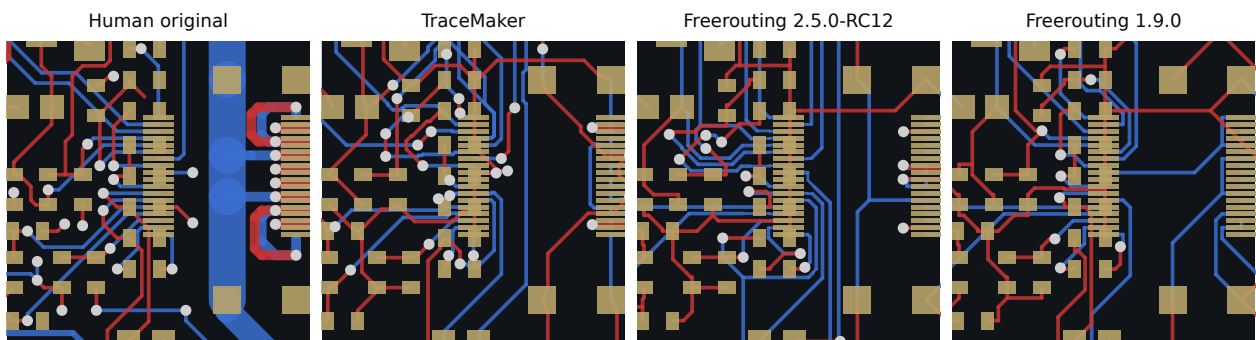
Figure 12: The same 22 mm window, centred on the densest pad area, in each result.
