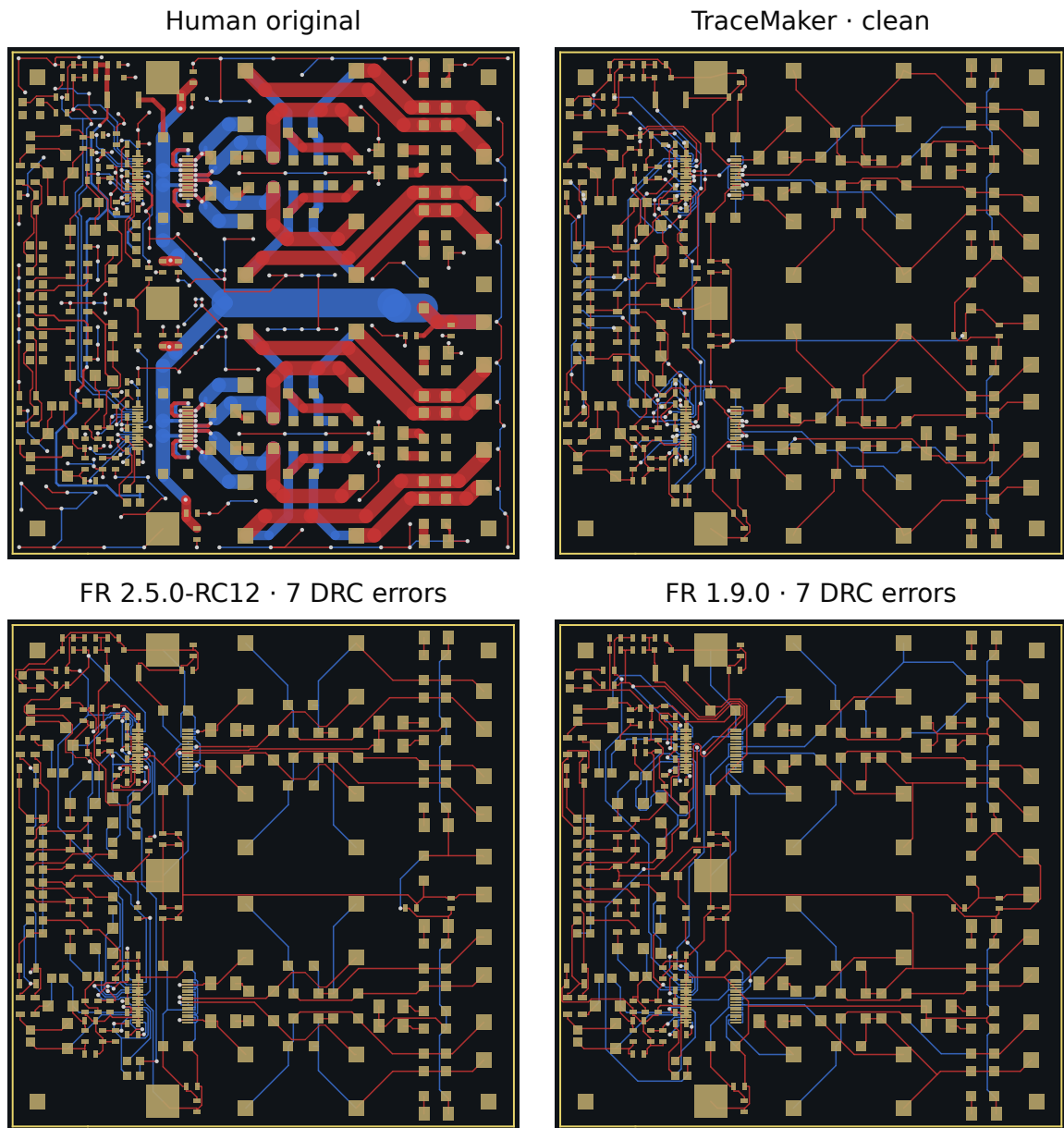
Figure 11: AmpOne routed four ways. The human design uses very wide power tracks; none of the routers does, because the board's net classes do not ask for them.
