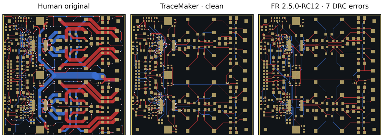
Figure 11: AmpOne routed three ways. The human design uses very wide power tracks; neither router does, because the board’s net classes do not ask for them.
