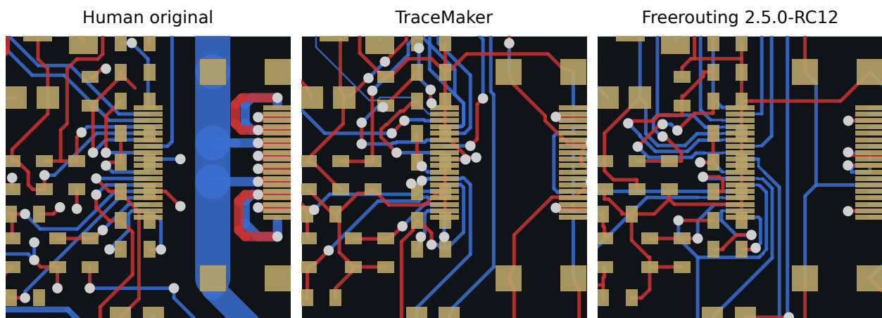
Figure 12: The same 22 mm window, centred on the densest pad area, in each result.
