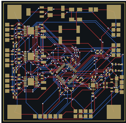
Routed: 1328 segments, 210 vias
