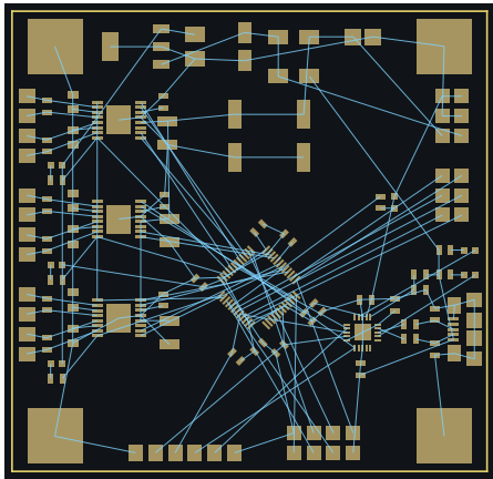
Input: pads and airwires
