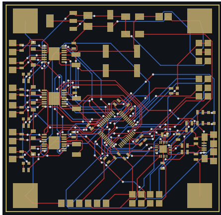
Routed: 918 segments, 164 vias
