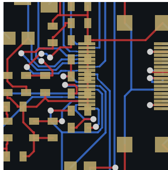
Freerouting 2.5.0-RC12
