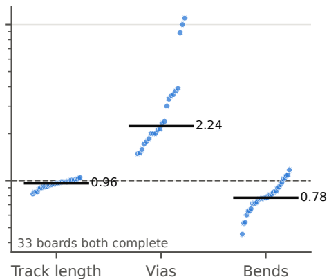
TraceMaker / FR 1.9.0
