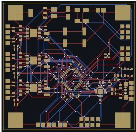
Routed: 807 segments, 136 vias
